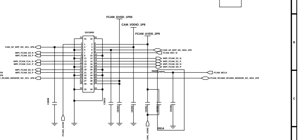
FRONT_32M CAMERA (30PIN)
