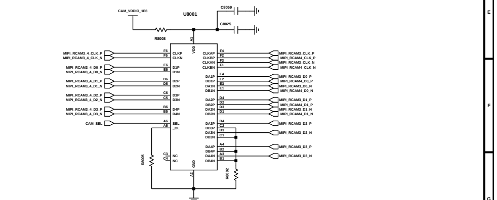
MIPI SWITCH (RCAM3,RCAM4)
